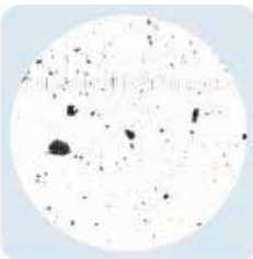
NAS 12 ISO 23/21/18 Typically New Oil as delivered in new certified mild steel 250 ltr barrels
