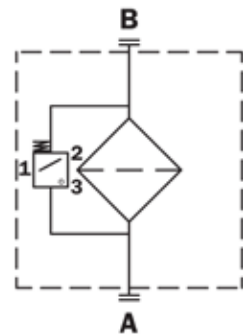
Circuit symbol
