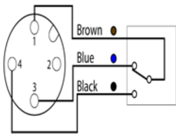
Connection diagram
